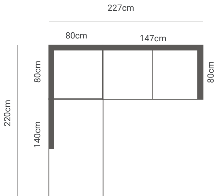
DRAWING 7 1 x 140 cm open-end w/A arm left 1 x 90° corner module 1 x 2,5 seat module w/A arm right
