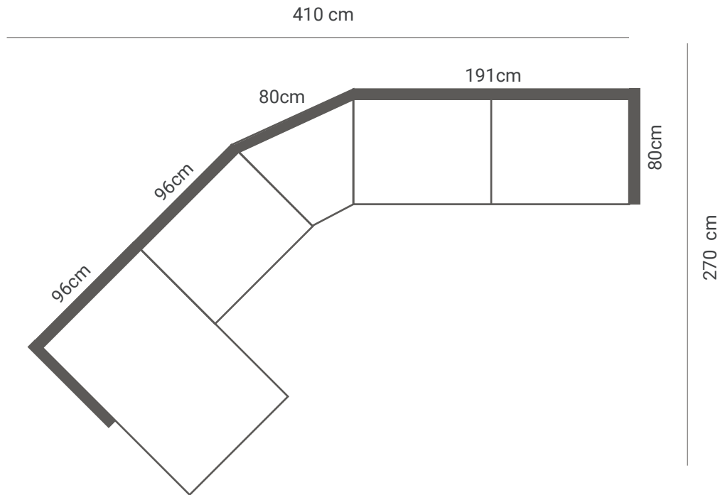
DRAWING 6 1 x 96 cm chaiselong w/A arm left 1 x 1,5 seat module w/out arms 1 x 45° corner module 1 x 3 seat module 2 cushions w/A arm right
